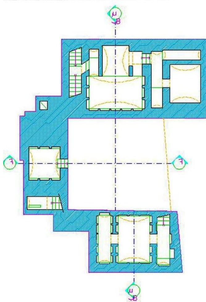
Basement Plan
